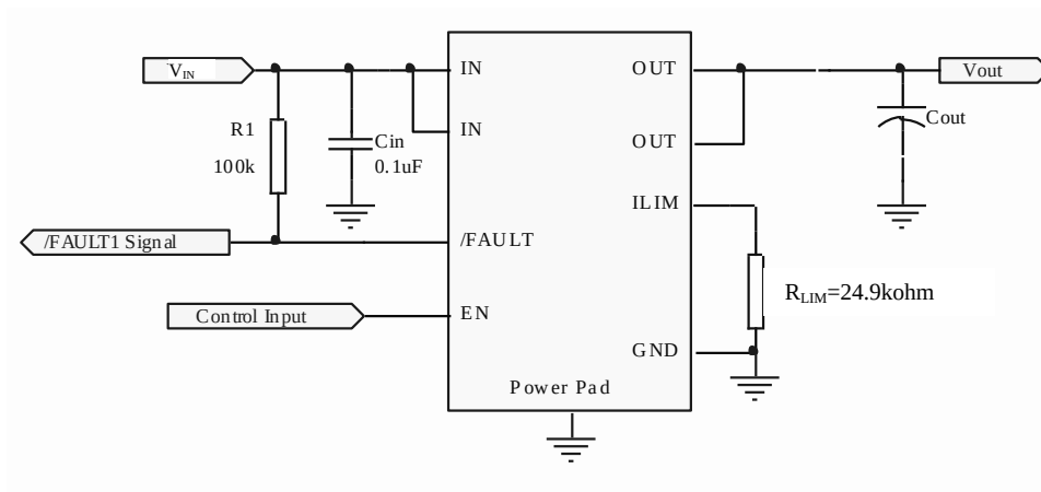
Figure 3 Typical Characteristics Reference Schematic
