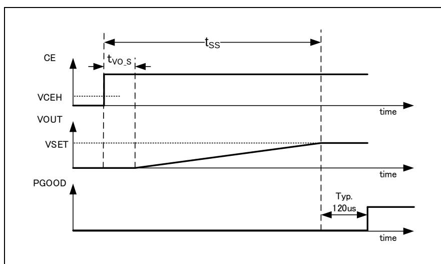
Soft-start Sequence
