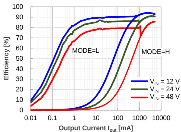
R1260S023A , V_{IN} = 12 V / 24V / 48 V , MODE = "High / Low" , V_{OUT} = 3.3 V
