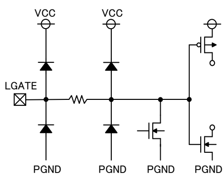
&lt; LGATE Pin &gt;
