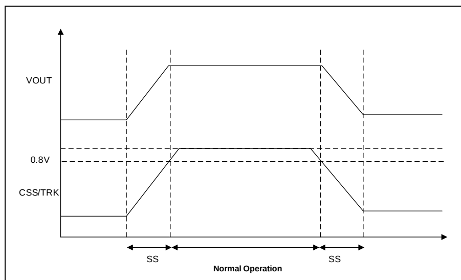
Tracking Sequence
