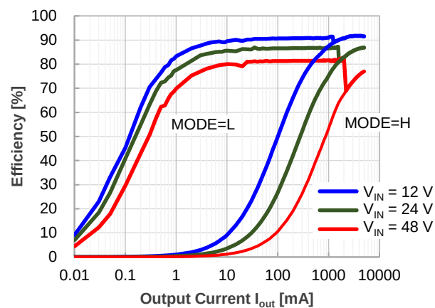
R1260S023A , V_{IN} = 12 V / 24V / 48 V , MODE = "High / Low" , V_{OUT} = 3.3 V
