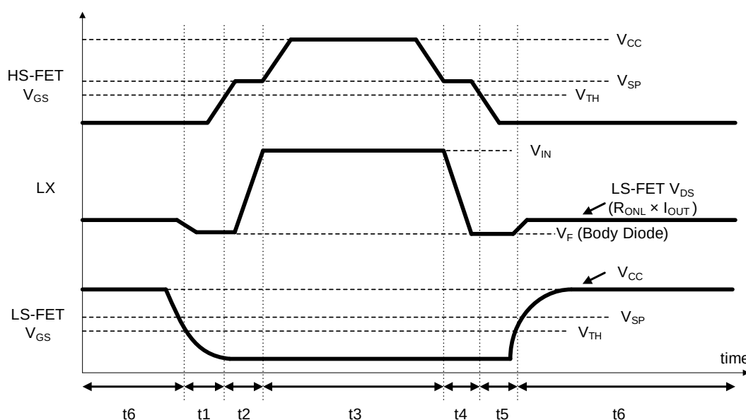
DC / DC Converter Basic Switching Timing Chart
