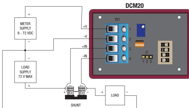
Figure 4. High-side current measurement, independent meter supply
