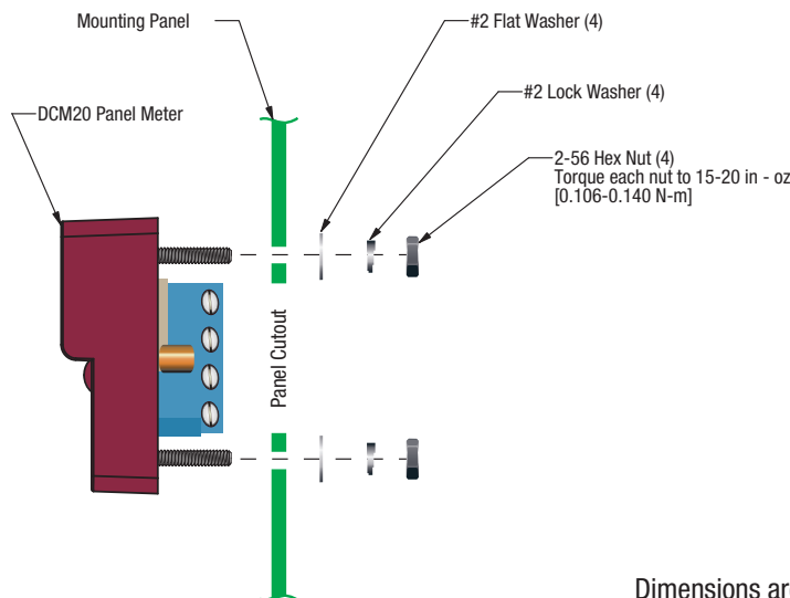
Figure 7. Panel installation
