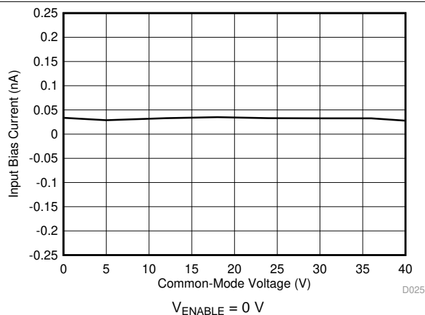
Figure 15. Input Bias Current vs Common-Mode Voltage (Shutdown)
