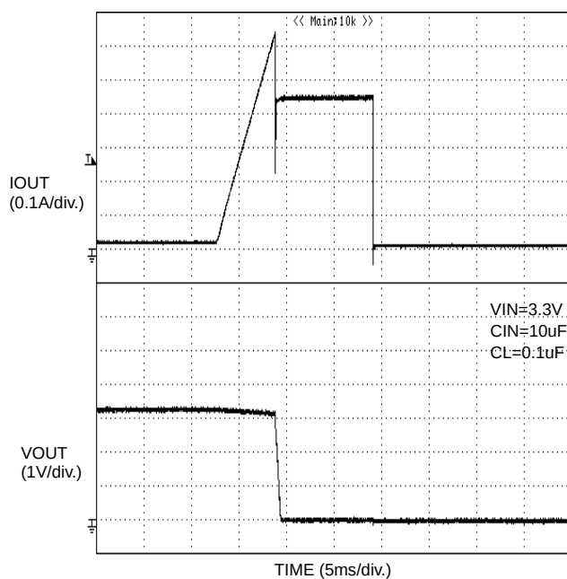
Figure 34. Current limit response Ramped load (1A/10ms) (BD2202G)
