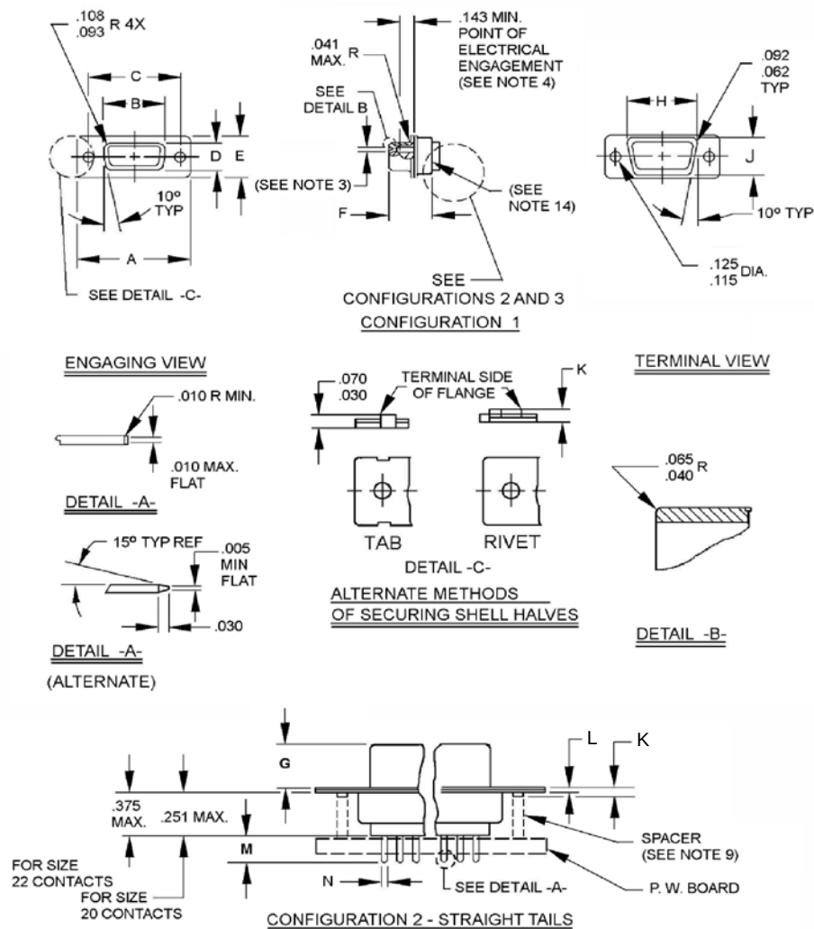
FIGURE 1. Shell, receptacle, printed wiring board type.
