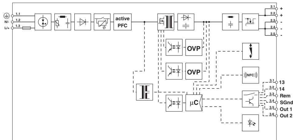
Figure 7 Block diagram
