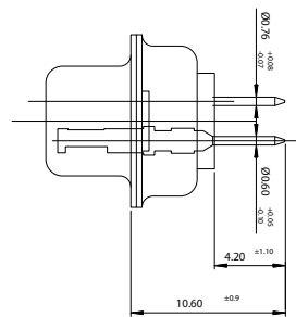
Straight PC tail contacts Z / OL3
