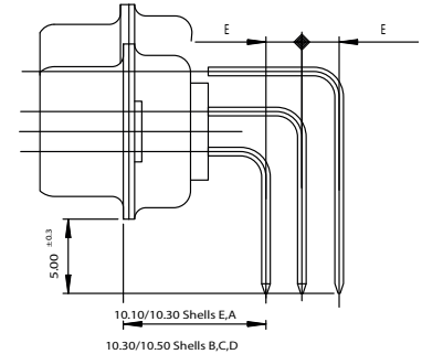
90° PC tail contacts without bracket 1A0N / 2A0N / 1B0N / 2B0N
