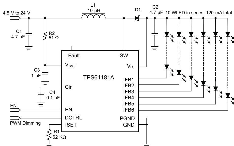
TPS61181A Typical Application
