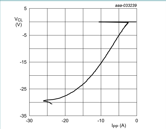
Fig. 6. Dynamic resistance with negative clamping; typical values Transmission Line Pulse (TLP); t p = 100 ns; t r = 1 ns
