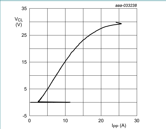
Fig. 5. Dynamic resistance with positive clamping; typical values Transmission Line Pulse (TLP); t p = 100 ns; t r = 1 ns
