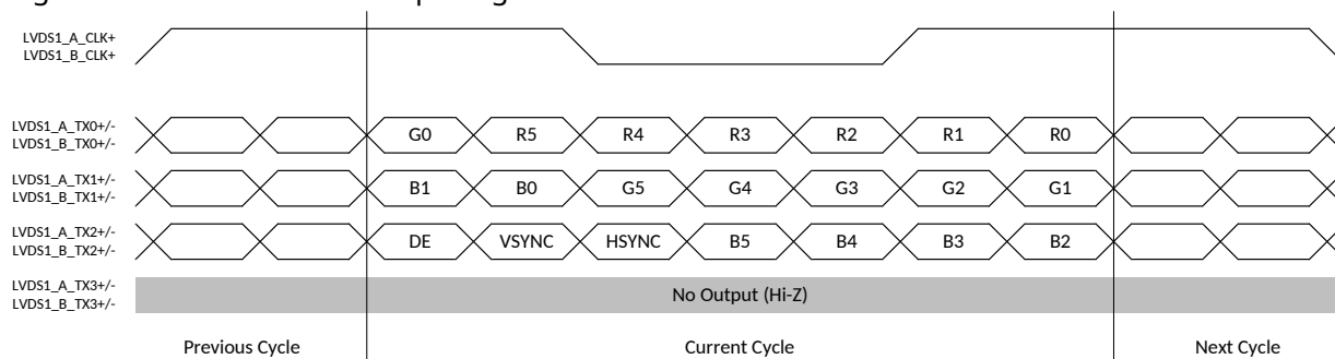
Figure 10: 18-bit Mode
