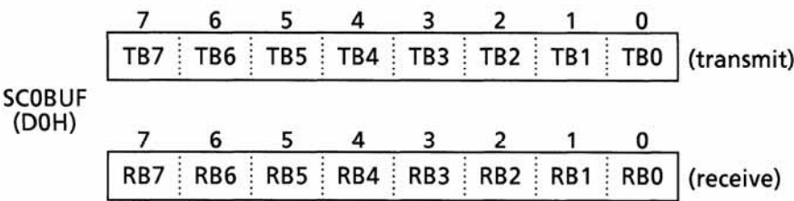
Figure 3.10.5 Serial Transmit/Receive Register (SC0BUF, Channel 0)
