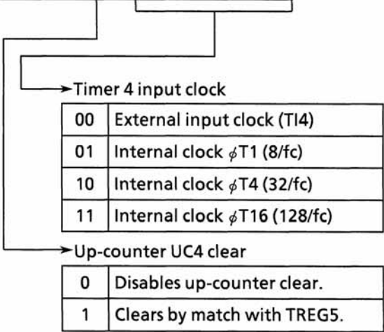
Figure 3.9.5 16-Bit Timer Mode Control Register (T4MOD) (1/2)
