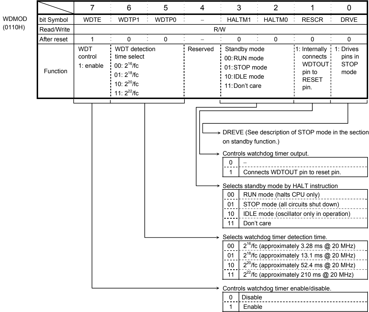
Figure 3.13.4 Watchdog Timer Mode Register
