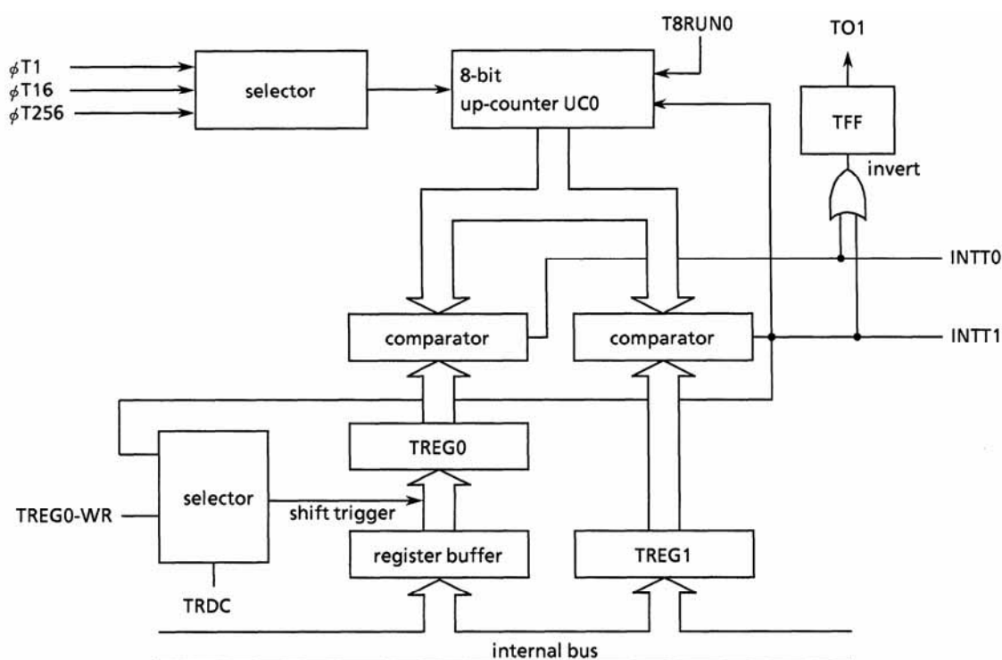
Figure 3.8.13 8-Bit PPG Output Mode Block Diagram
