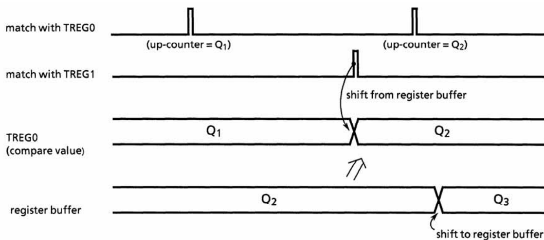
Register Buffer Operation
