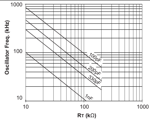
Figure 4. UCC2813-[3,5]-Q1: Oscillator Frequency vs R_T and C_T
