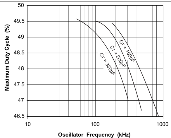
Figure 6. UCC2813-[1,4,5]-Q1: Maximum Duty Cycle vs Oscillator Frequency
