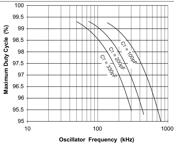
Figure 5. UCC2813-[0,2,3]-Q1: Maximum Duty Cycle vs Oscillator Frequency
