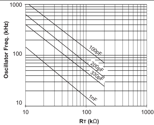
Figure 3. UCC2813-[0,1,2,4]-Q1: Oscillator Frequency vs R_T and C_T
