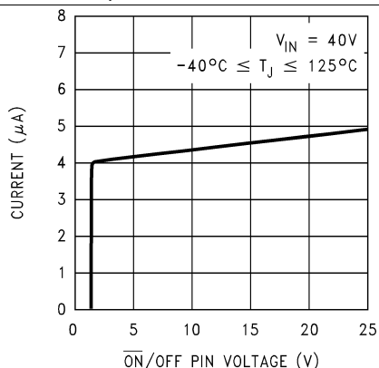
Figure 13. \overline{ON}/\overline{OFF} Pin Current (Sinking)
