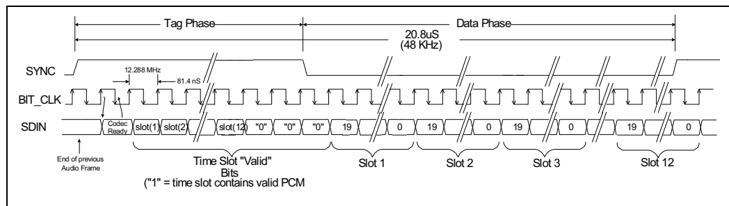
Figure 25. AC-Link Protocol
