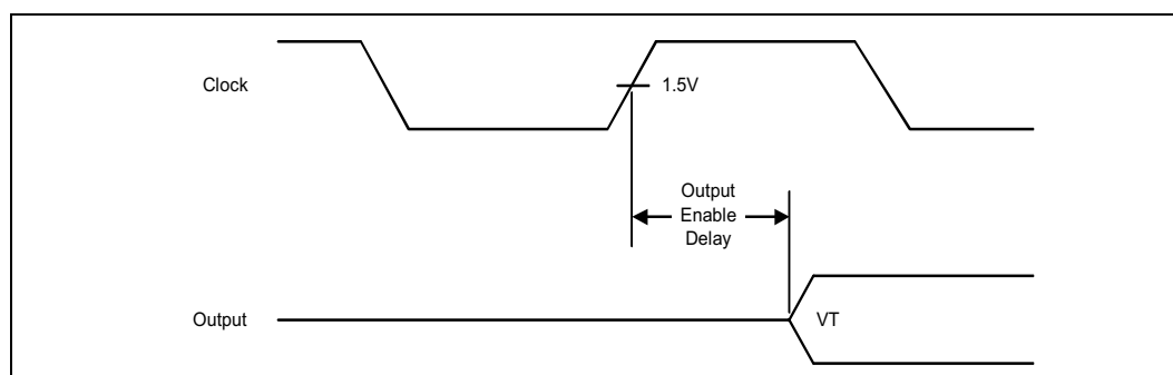
Figure 49. Output Enable Delay
