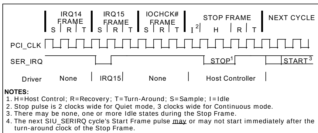
Figure 35. Stop Frame Timing with Host Using 17 SIU_SERIRQ Sampling Period
