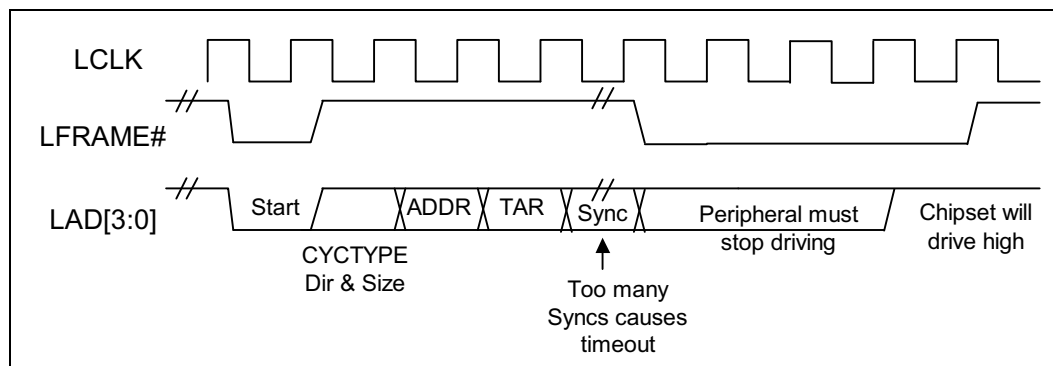
Figure 10. Abort Mechanism
