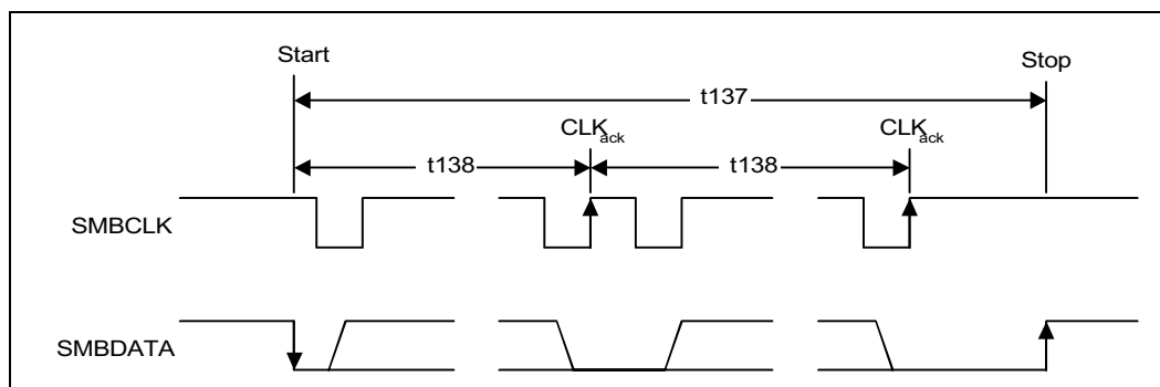
Figure 60. SMBus Timeout
