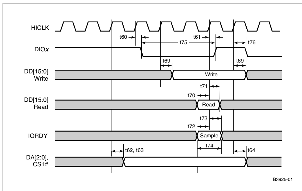
Figure 50. IDE PIO Mode
