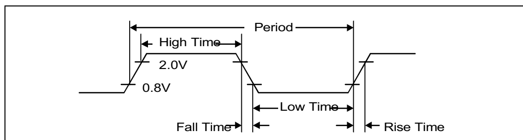
Figure 44. Clock Timing
