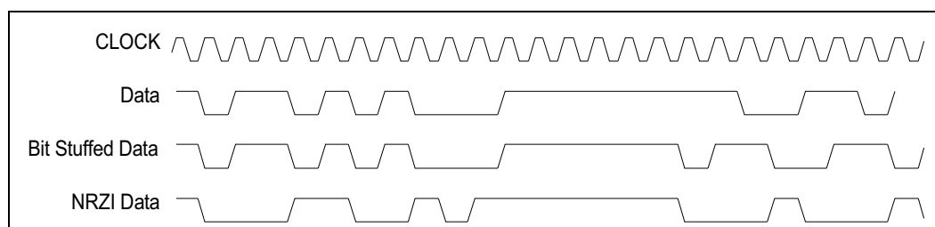
Figure 20. USB Data Encoding
