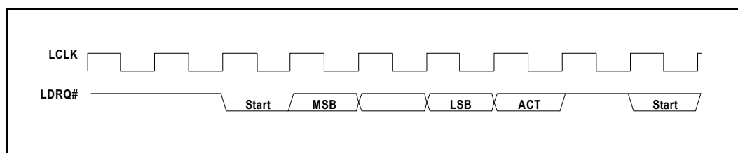
Figure 12. DMA Request Assertion Through LDRQ#
