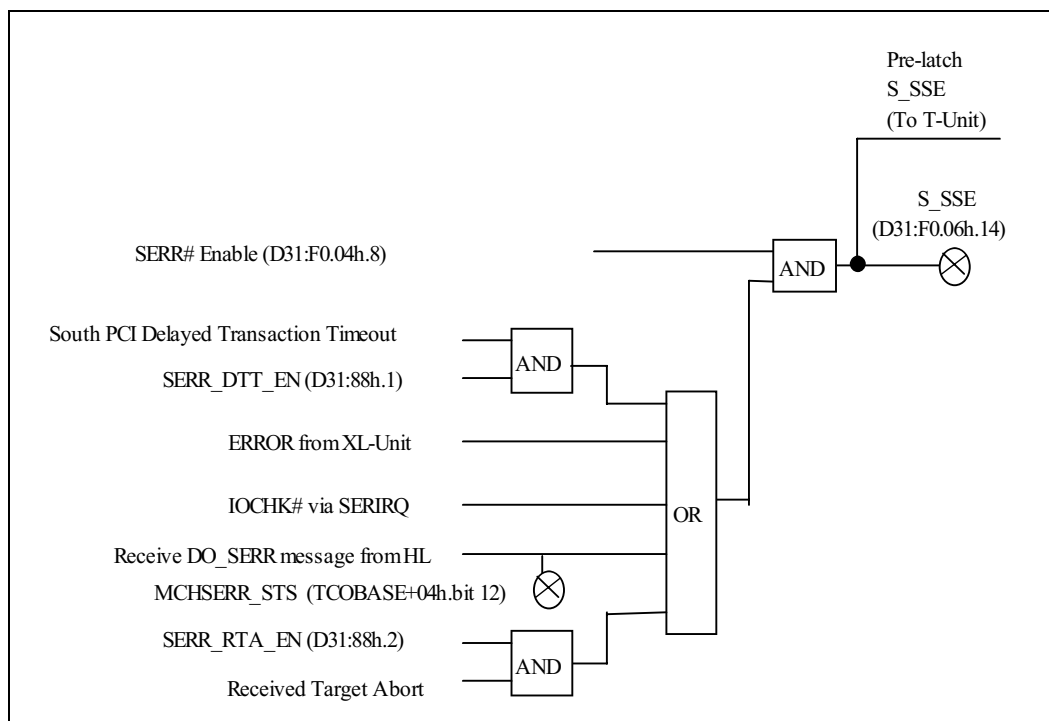
Figure 7. Secondary Status Register Error Reporting Logic
