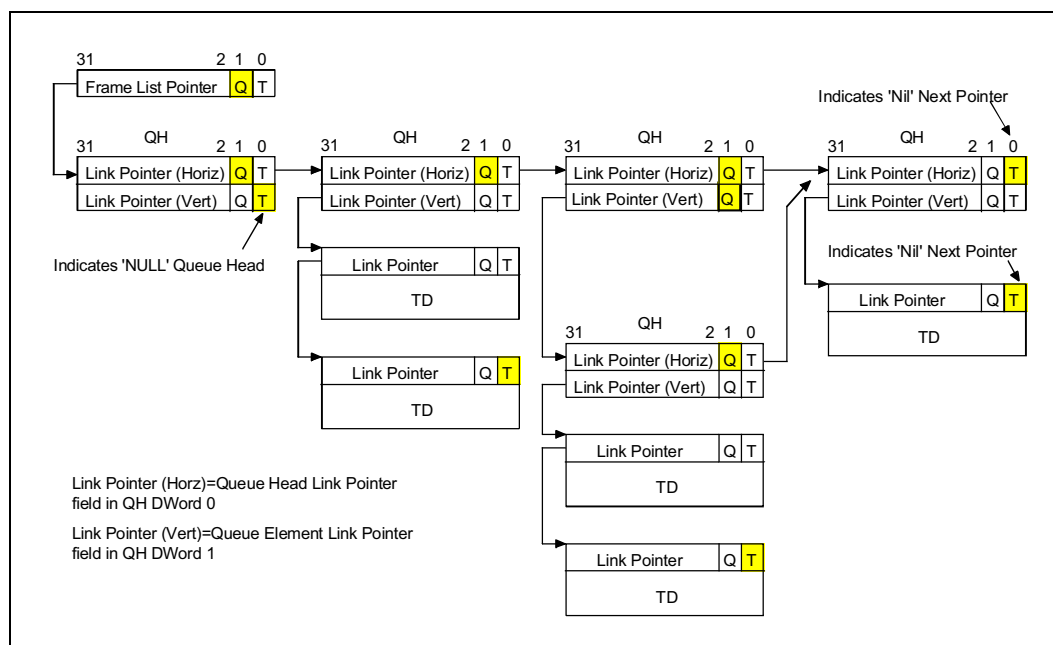
Figure 19. Example Queue Conditions
