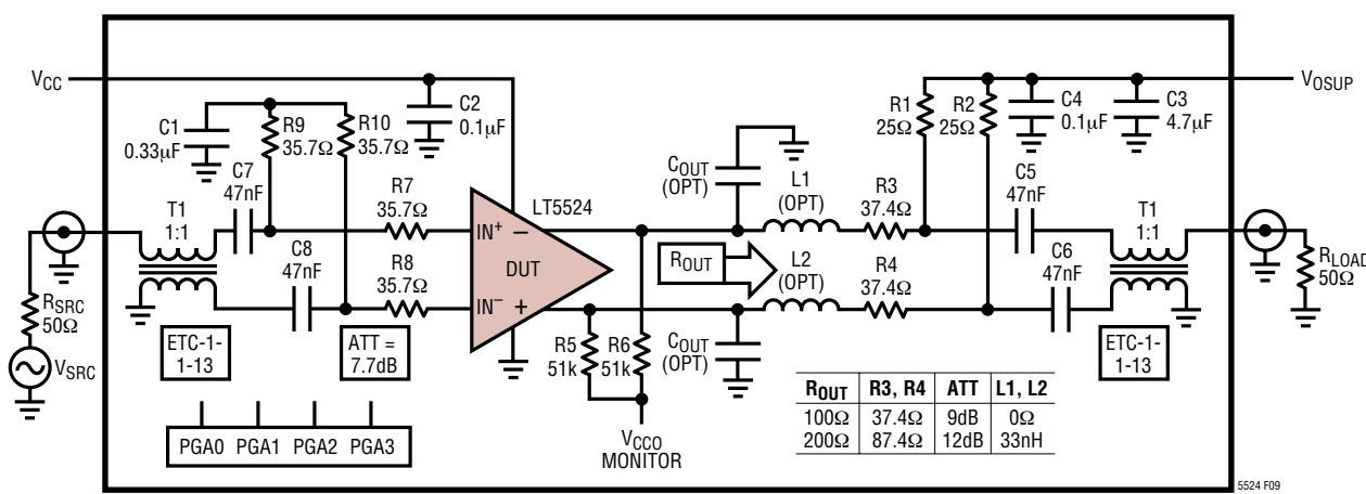
Figure 9. Characterization Board (Simplified Schematic)
