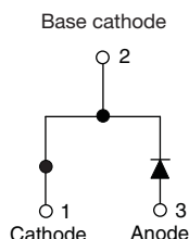
TO-247AD 2L
