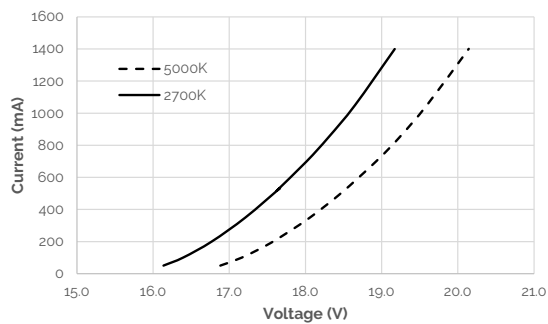
Figure 1: Forward Voltage vs. Forward Current, T_c = 25^\circ\text{C}
