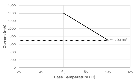
Figure 8: Derating Curve
