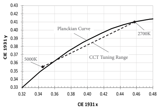
Figure 6: CCT Tuning Range, T_c = 85^\circ\text{C}
