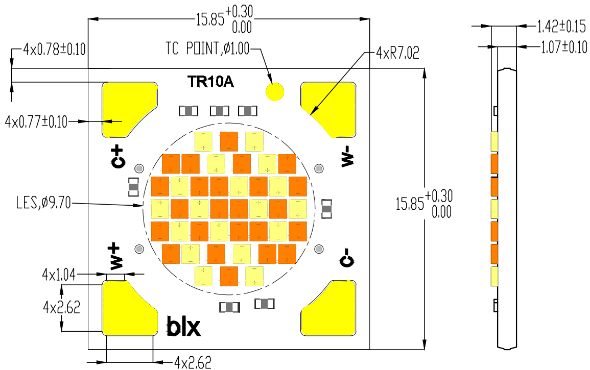
Figure 12: Drawing for Vesta Series Tunable White gmm LED Array
