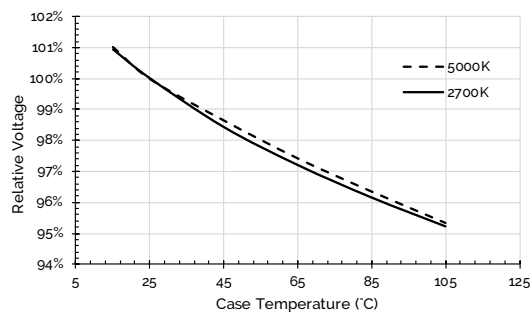
Figure 4: Forward Voltage vs. Case Temperature
