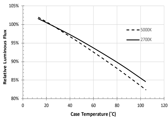
Figure 3: Relative Flux vs. Case Temperature
