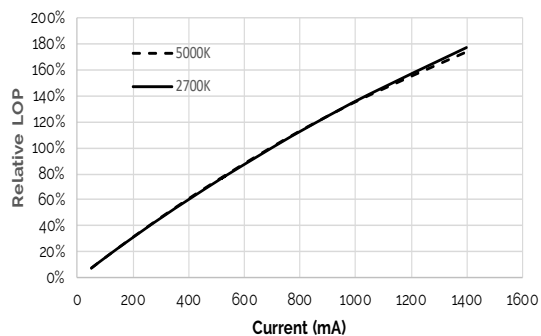
Figure 2: Relative Flux vs. Drive Current, T_c = 25^\circ\text{C}
