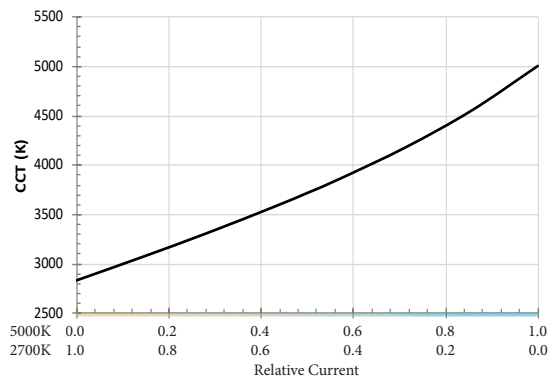
Figure 5: CCT vs. Current, T_c = 85^\circ\text{C}
