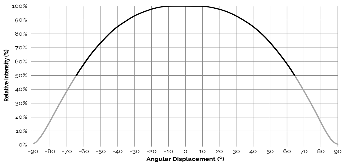
Figure 9: Typical Spatial Radiation Pattern
