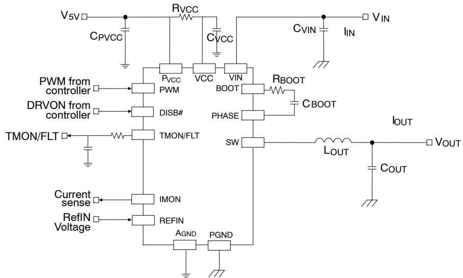
Figure 1. Application Schematic
