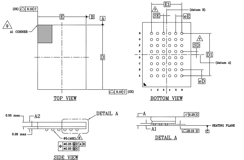
Figure 11. 48-ball VFBGA (6 × 8 × 1.0 mm) Package Outline, 51-85150
