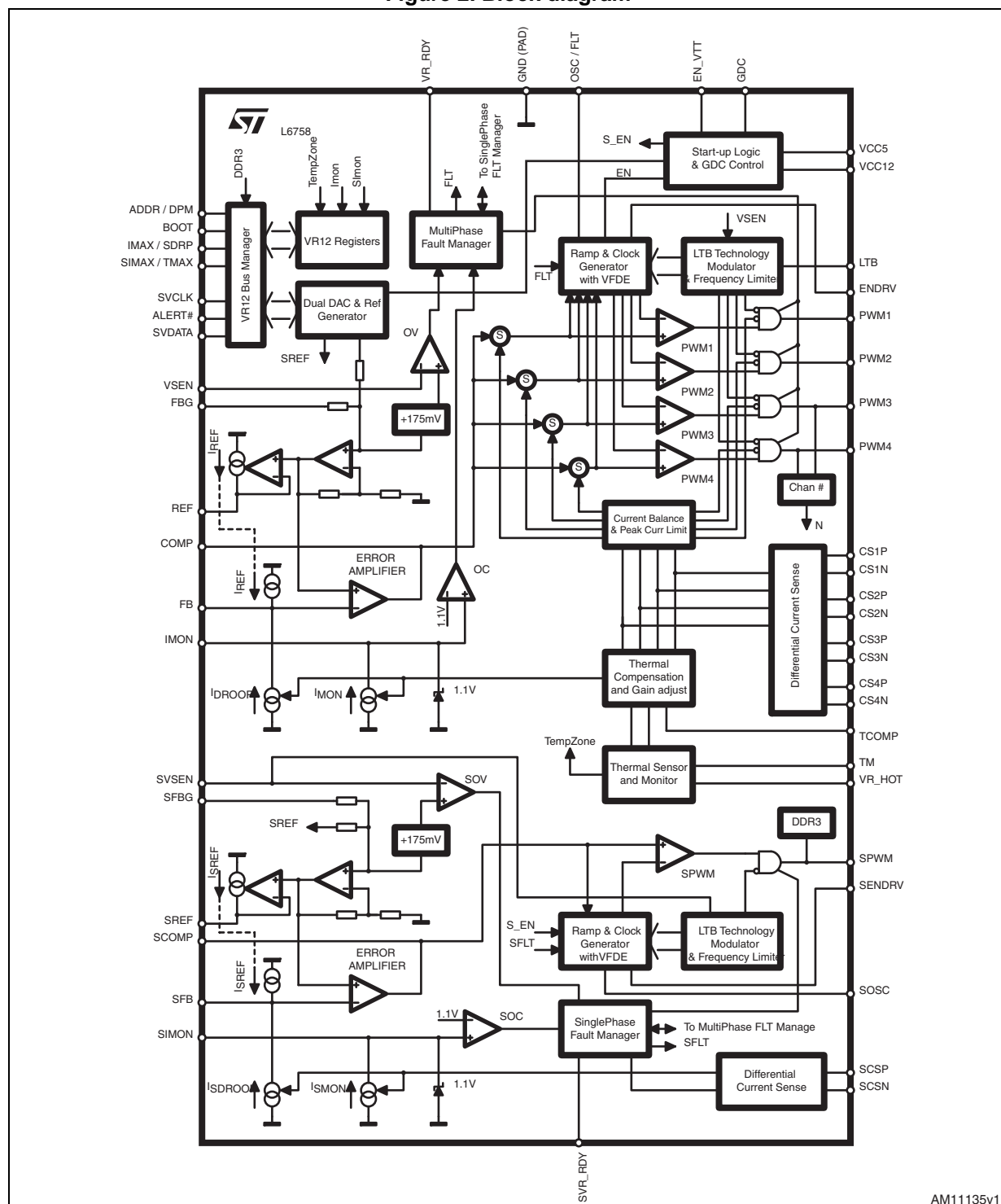
Figure 2. Block diagram
