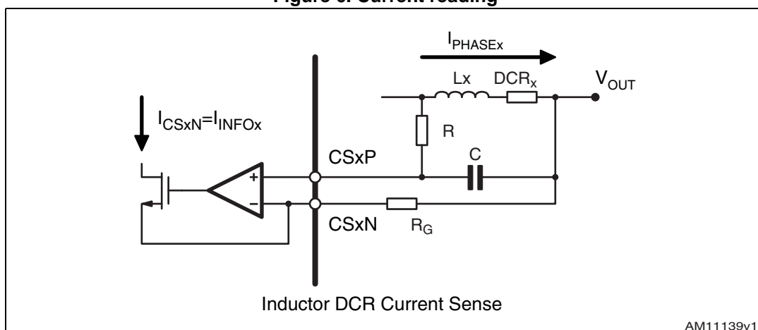
Figure 6. Current reading
