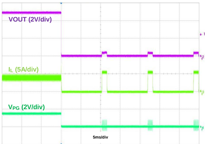
Figure 11. Output Short Protection with PG, I_{OUT} = 4\text{A}
