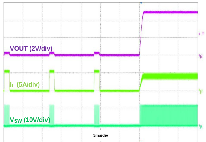
Figure 10. Output Short Recovery, I_{OUT} = 4\text{A}
