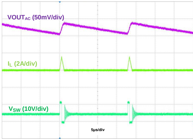
Figure 19. Output Voltage Ripple, V_{OUT} = 5\text{V} , I_{OUT} = 50\text{mA}
