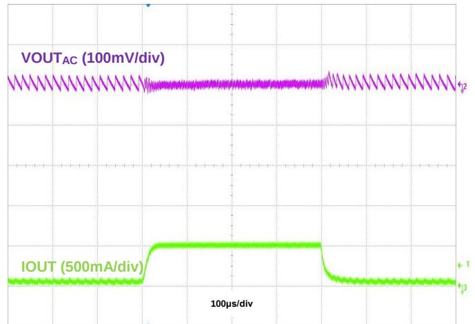
Figure 22. Load Transient, I_{OUT} = 50\text{mA} to 500\text{mA} to 50\text{mA}
