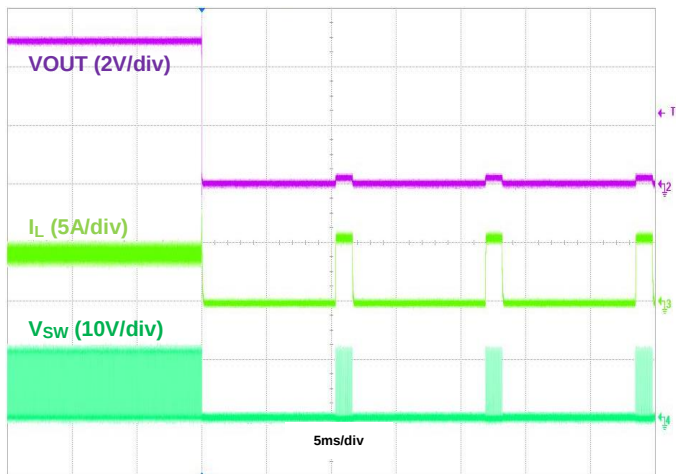
Figure 9. Output Short Protection, I_{OUT} = 4\text{A}
