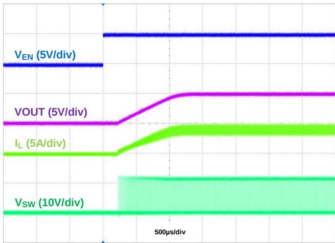
Figure 7. Startup Using EN, I_{OUT} = 4\text{A}
