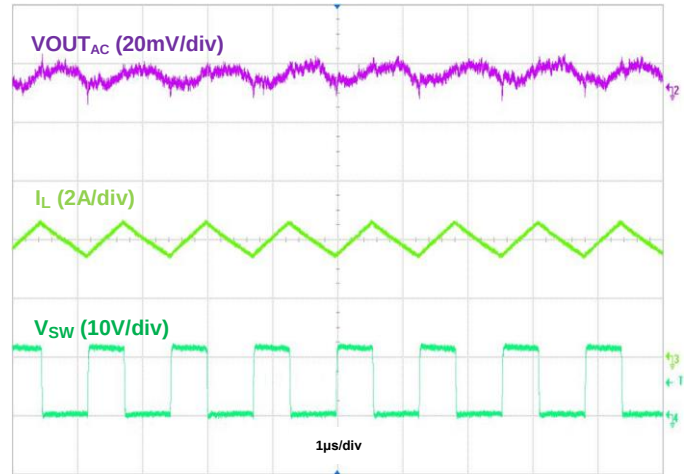
Figure 20. Output Voltage Ripple, V_{OUT} = 5\text{V} , I_{OUT} = 4\text{A}
