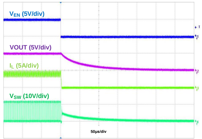
Figure 8. Shutdown Using EN, I_{OUT} = 4\text{A}
