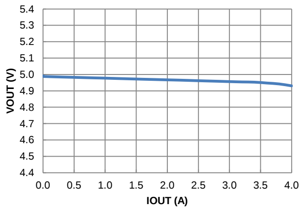
Figure 27. Load Regulation
