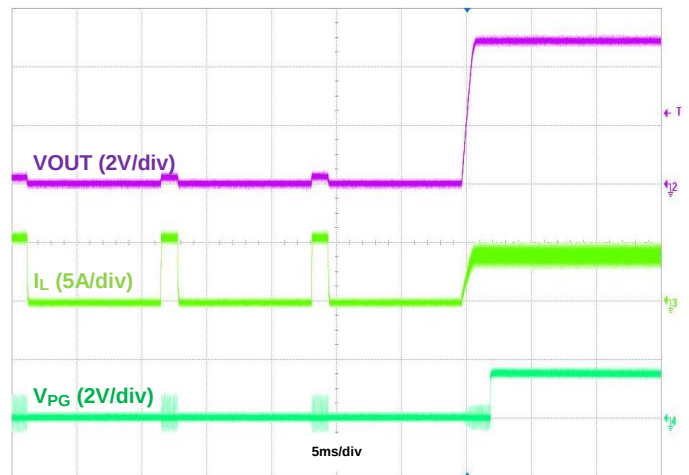
Figure 12. Output Short Recovery with PG, I_{OUT} = 4\text{A}
