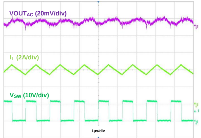
Figure 32. Output Voltage Ripple, V_{OUT} = 5\text{V} , I_{OUT} = 4\text{A}
