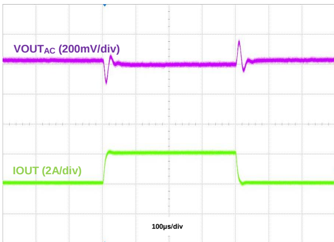
Figure 23. Load Transient, I_{OUT} = 2\text{A} to 4\text{A} to 2\text{A}
