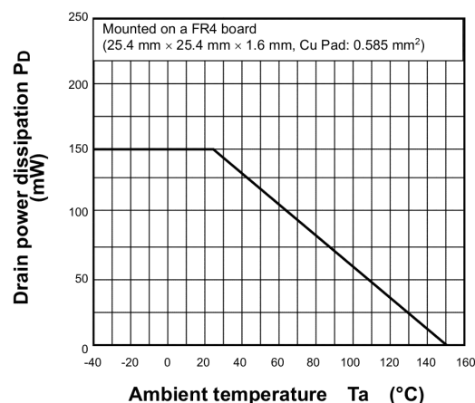
Fig. 7.12 P_D - T_a
