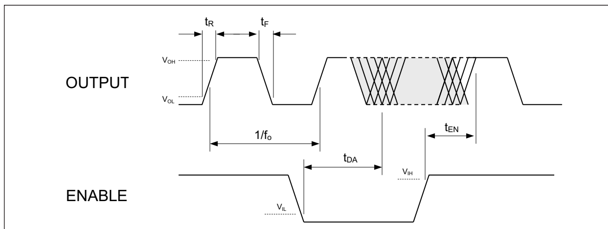
FIGURE 4-1: DSA613 Output Waveform.
