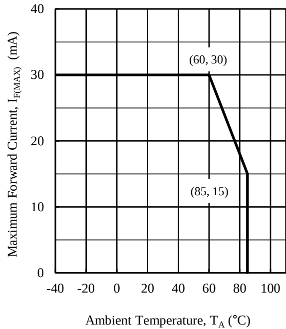
Figure 1. I_{F(MAX)} vs. T_A
