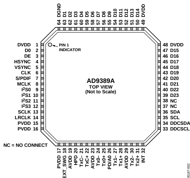
Figure 2. Pin Configuration
