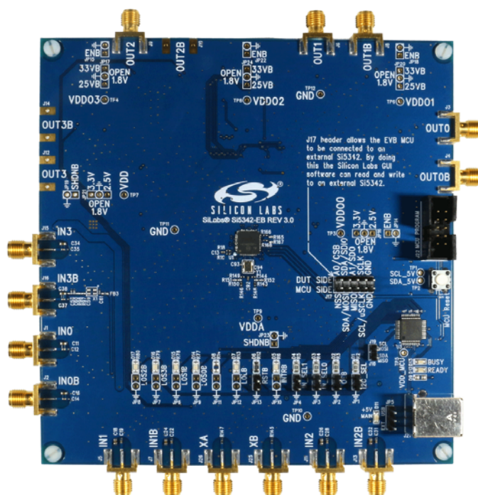
Figure 1. Si5342 Evaluation Board
