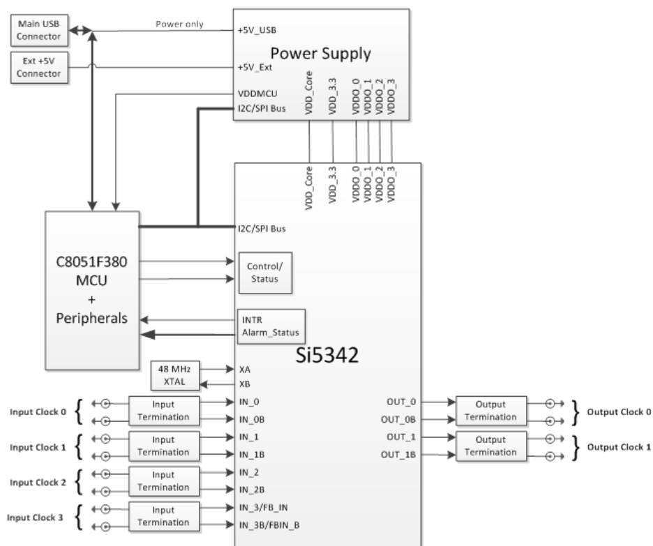
Figure 2. Si5342-EVB Functional Block Diagram
