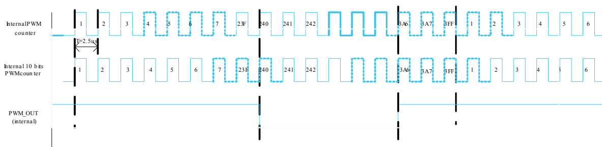
Figure 16. Resulting waveform 4
