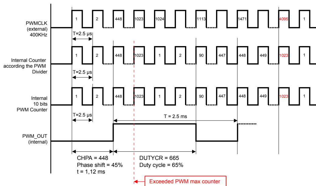
Figure 14. Resulting waveform 2
