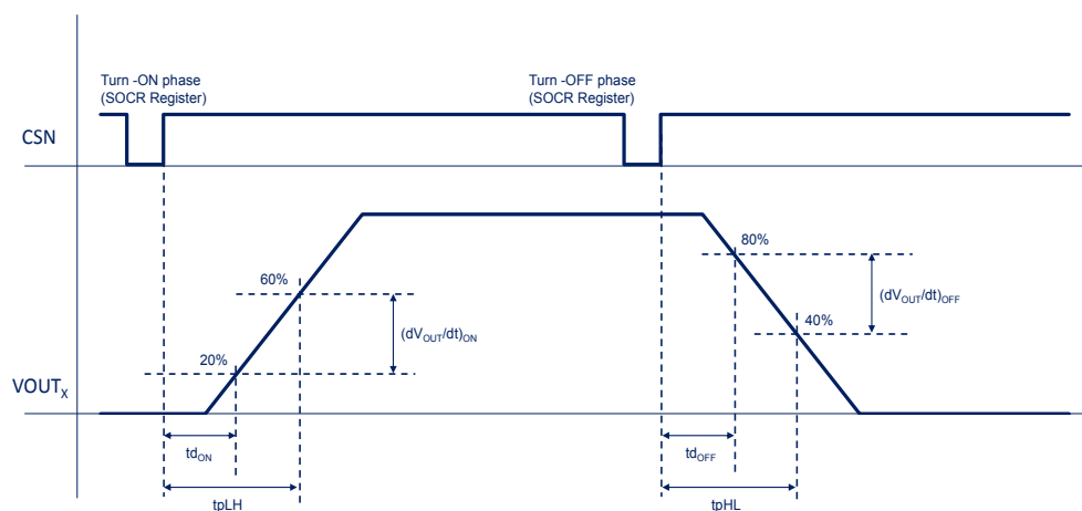
Figure 34. Switching characteristics
