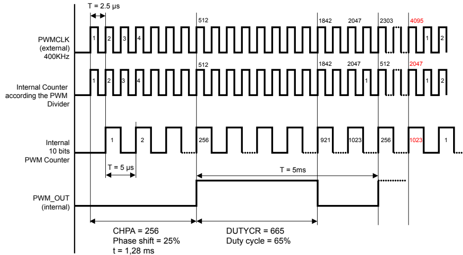
Figure 13. Resulting waveform 1
