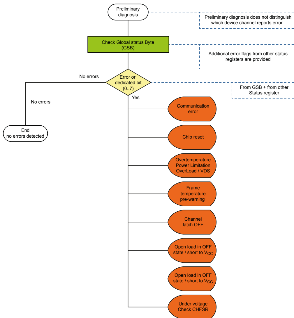
Figure 25. Status registers
