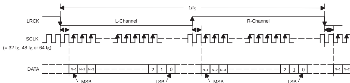
Figure 26. I^2S Format
