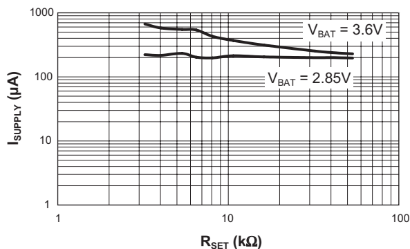
Operating Supply Current vs. R_{SET} ( V_{IN} = 5V )
