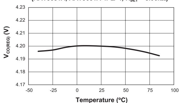
Constant Regulated Output Voltage vs. Temperature (AAT3681A, AAT3681A-1/-2/-4; R_{SET} = 8.06k\Omega )
