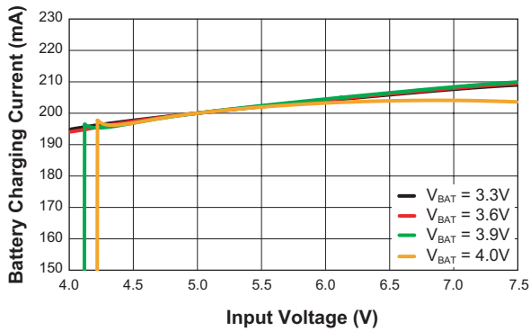
Battery Charging Current vs. Input Voltage (AAT3681A-4.1 and AAT3681A-5 only; V_{CO(REG)} = 4.1V )
