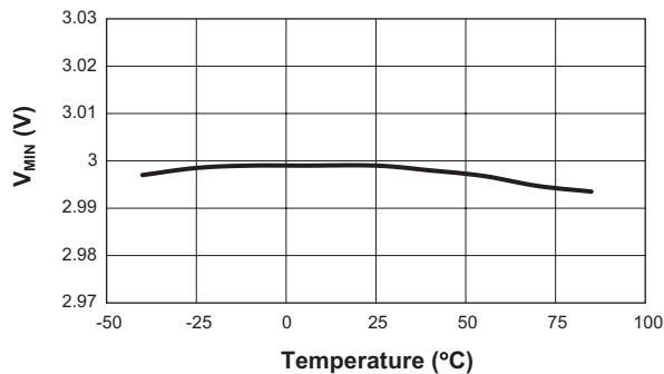
Preconditioning Threshold Voltage vs. Temperature ( R_{SET} = 8.06k\Omega ; AAT3681A, AAT3681A-2, and AAT3681A-5 Only)
