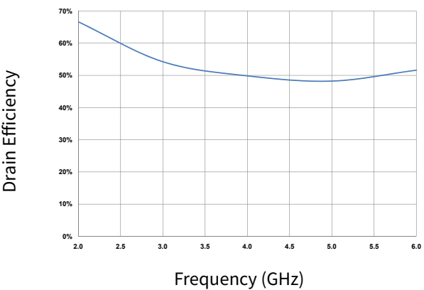
Figure 9. Drain Efficiency vs Frequency of the CGH40006S in the CGH40006S-AMP1 at P_{IN} = 32\text{ dBm} , V_{DD} = 28\text{ V}
