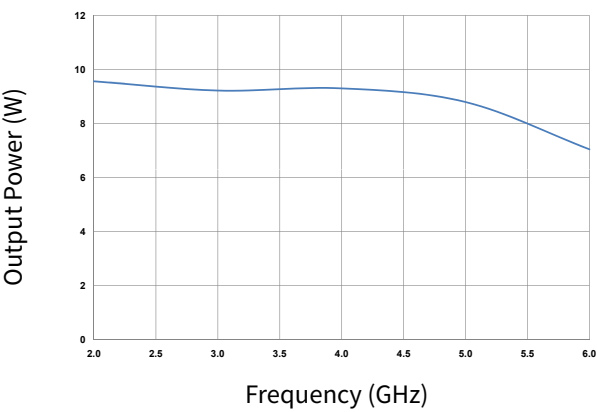
Figure 8. Output Power vs Frequency of the CGH40006S in the CGH40006S-AMP1 at P_{IN} = 32\text{ dBm} , V_{DD} = 28\text{ V}
