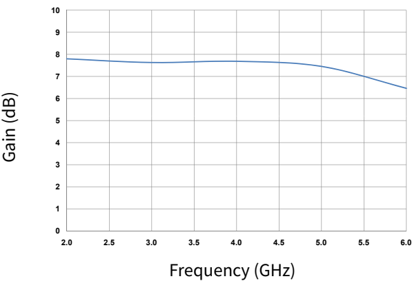
Figure 7. Power Gain vs Frequency of the CGH40006S in the CGH40006S-AMP1 at P_{IN} = 32\text{ dBm} , V_{DD} = 28\text{ V}
