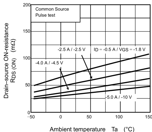
Fig. 8.6 R_{DS(ON)} - T_a
