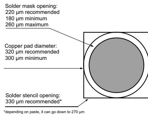
Figure 20. Footprint - 5 mils stencil - solder mask defined
