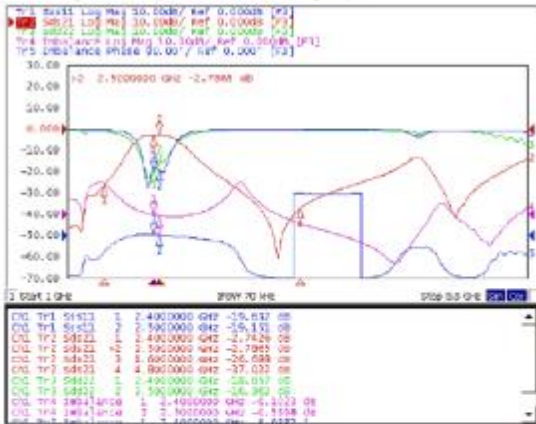
2012 / 2.45GHz Bluetooth/WLAN Balanced Filter CBA4711 713 67 2453K
