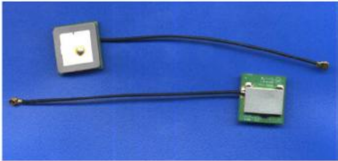
1919 / 1.575GHz GPS Ceramic Active Antenna CAN 431343793158 1B
