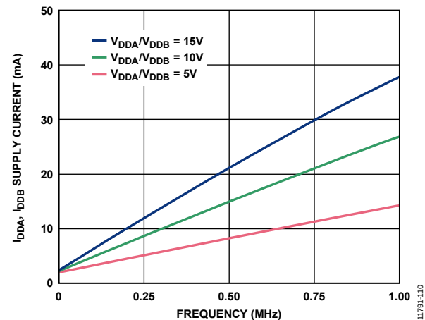
Figure 10. Typical I_{ODA} , I_{ODB} Supply Current vs. Frequency with 2 nF Load
