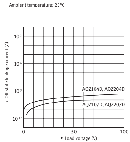
11-2. Off state leakage current vs. load voltage characteristics
