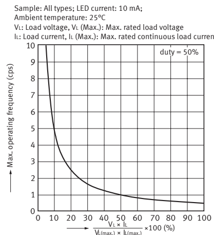
12. Max. operating frequency vs. load voltage and load current characteristics
