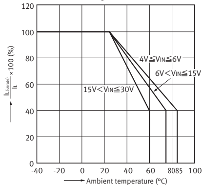
2-3. Load current vs. ambient temperature characteristics in adjacent mounting-
