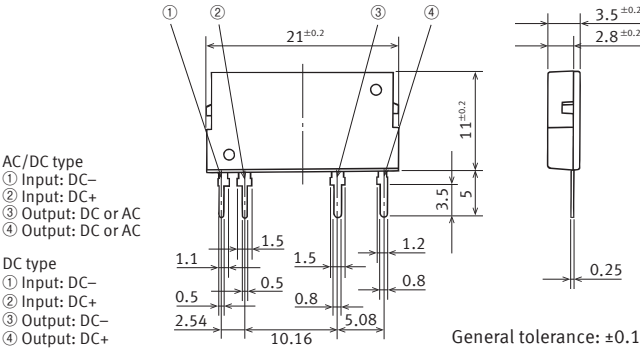
External dimensions
