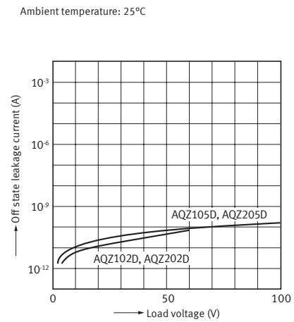
11-1. Off state leakage current vs. load voltage characteristics
