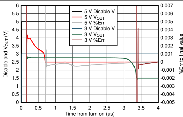
Single-supply, DC input to produce midscale output (simulation) Figure 6-53. Gain of 6-V/V Turn-On Time to Final DC Value at Midscale
