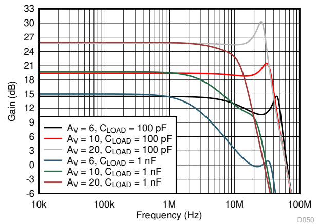
See Figure 7-6 and Table 8-1 2-kΩ parallel load to C_{LOAD} Figure 6-50. Small-Signal Response Shapes vs C_{LOAD} With Recommended R_{OUT}
