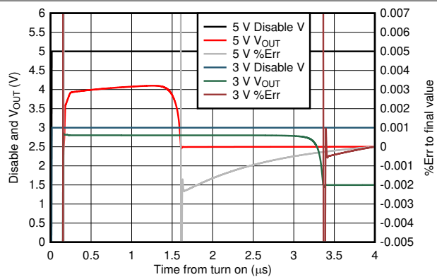
Single-supply, DC input to produce midscale output (simulation) Figure 6-54. Gain of 10-V/V Turn-On Time to Final DC Value at Midscale
