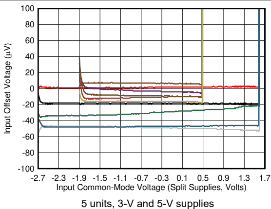
Figure 6-59. Input Offset Voltage vs Input Common- Mode Voltage
