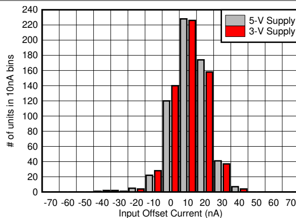
Figure 6-44. Input Offset Current Distribution
