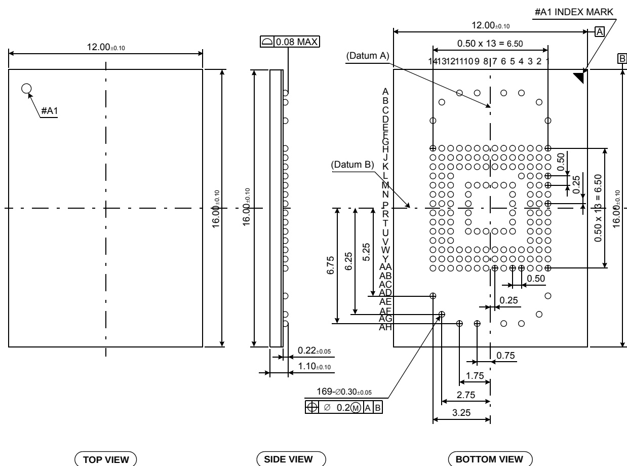
Figure 5. 12mm x 16mm x 1.2mm Package Dimension
