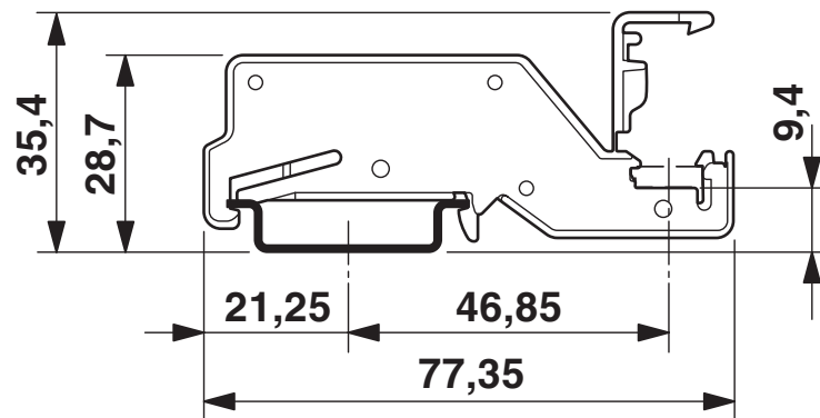
Dimensional drawing
