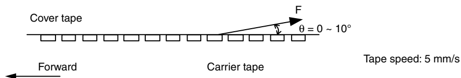
Fig. 10 Tape Separation
