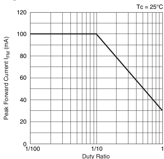
Fig. 2 Peak Forward Current vs. Duty Ratio
