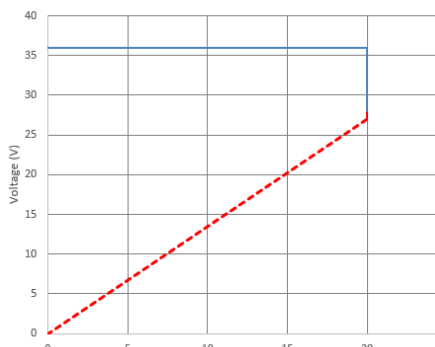
PQU650M-36P; Constant Current OCP
