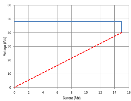
PQU650M-48P; Constant Current OCP
