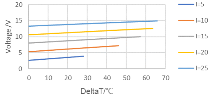
Performance Curves at T_h=27^\circ\text{C}
