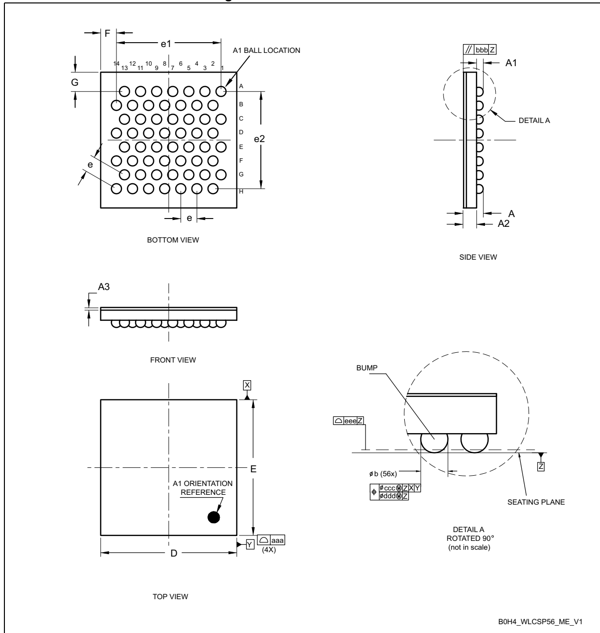
Figure 68. WLCSP56 - Outline
