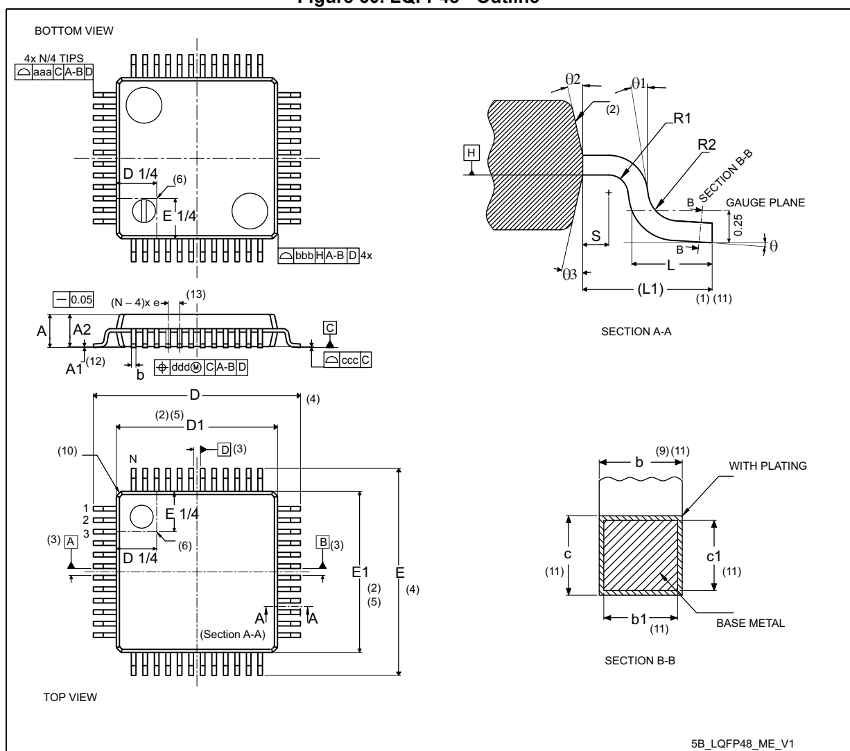
Figure 60. LQFP48 - Outline (15)
