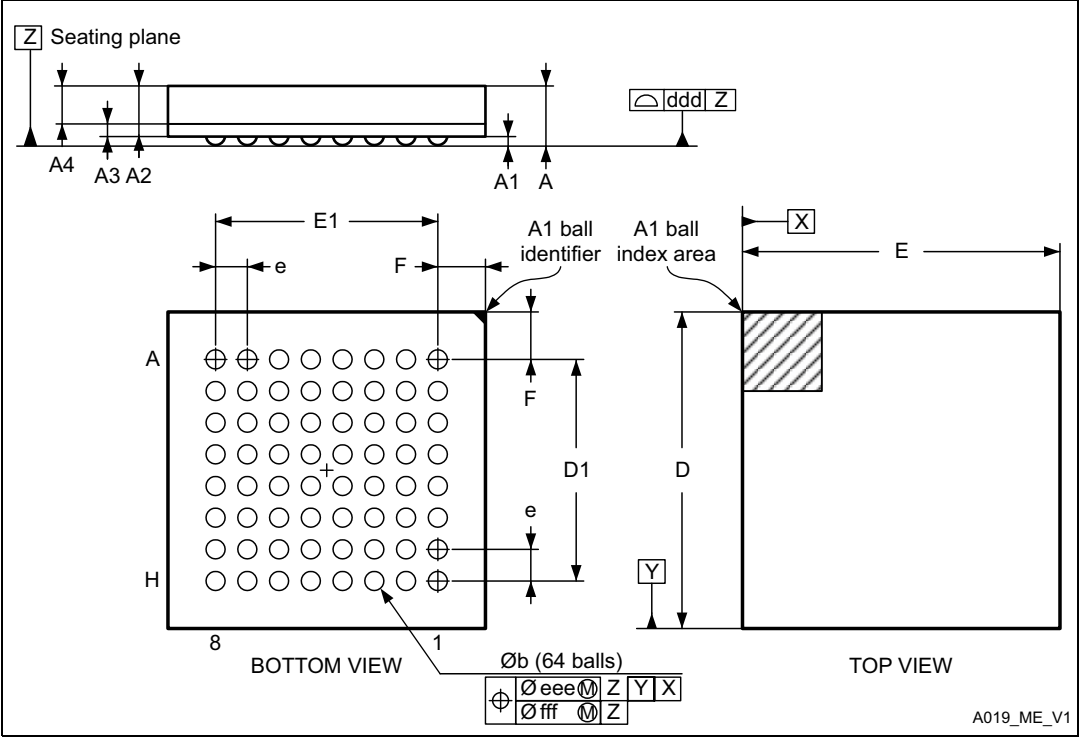
Figure 66. UFBGA64 – Outline
