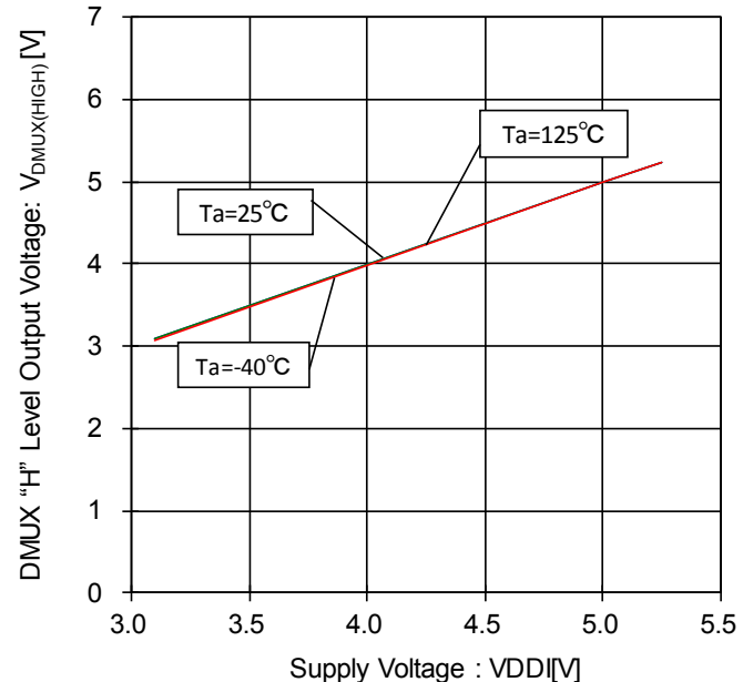
Figure 96. DMUX "H" Level Output Voltage- Voltage Characteristic ( I_{SOURCE}=200\mu\text{A} )
