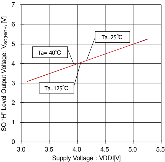
Figure 90. SO "H" Level Output Voltage- Voltage Characteristic ( I_{SOURCE}=200\mu A )
