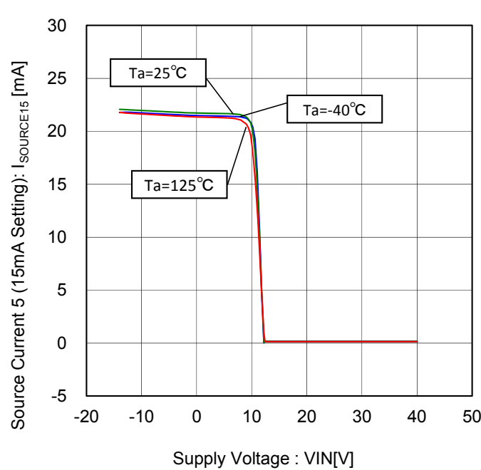
Figure 66. Source Current 5- Voltage Characteristic (15mA Setting)
