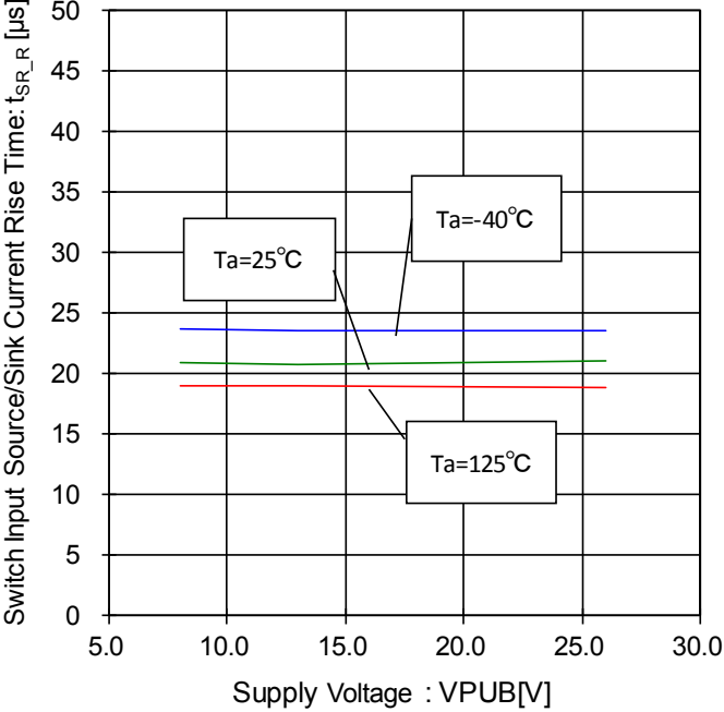
Figure 118. Switch Input Source/Sink Current Rise Time-Voltage Characteristic (FSQ="0", FSQZ/A/B="0", 10mA Setting, Load Resistance=100 \Omega )
