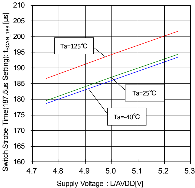
Figure 114. Switch Strobe Time- Voltage Characteristic (187.5µsSetting)
