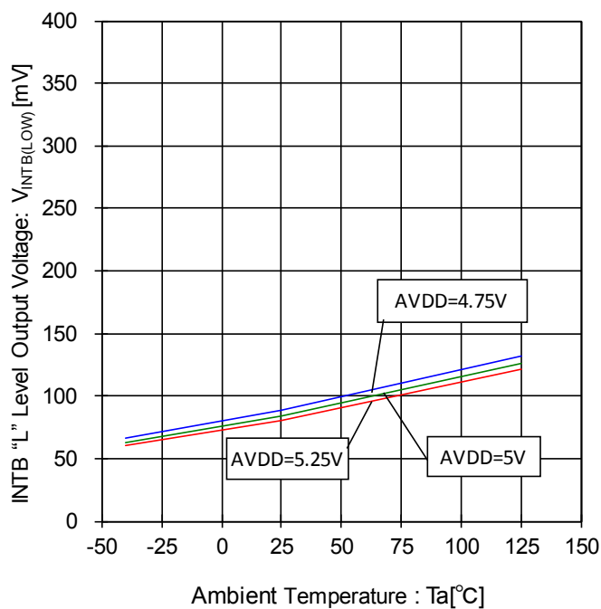
Figure 103. INTB "L" Level Output Voltage- Temperature Characteristic ( I_{SINK}=1.0\text{mA} )
