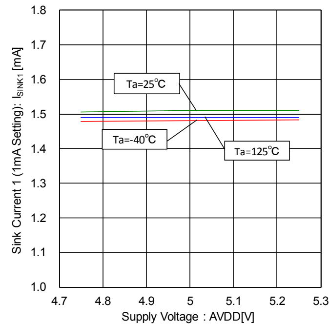
Figure 36. Sink Current 1- Voltage Characteristic (1mA Setting, 8V external supply)
