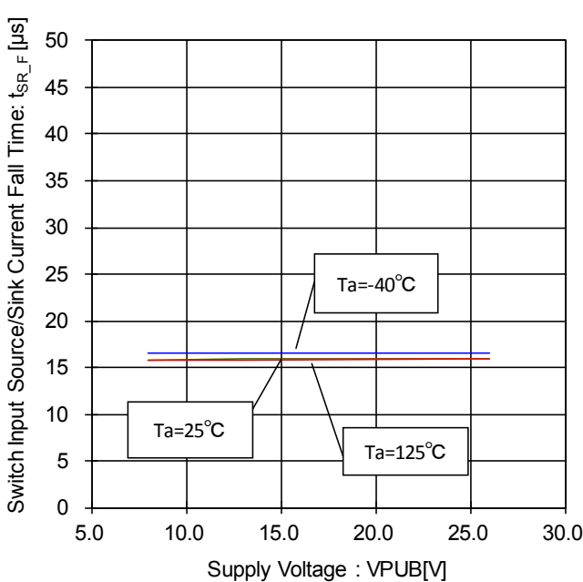
Figure 120. Switch Input Source/Sink Current Fall Time-Voltage Characteristic (FSQ="0", FSQZ/A/B="0", 10mA Setting, Load Resistance=100 \Omega )
