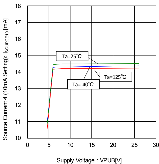
Figure 56. Source Current 4- Voltage Characteristic (10mA Setting, 0V external supply)
