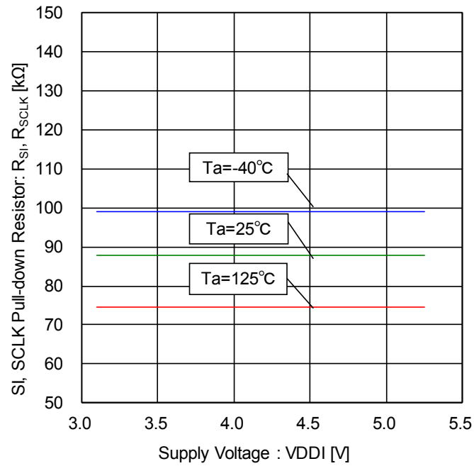
Figure 86. SI, SCLK Pull-down Resistor- Voltage Characteristic
