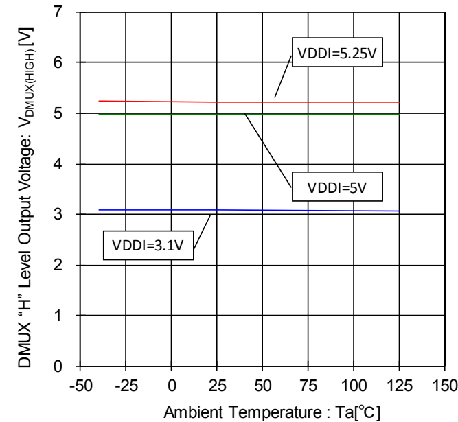
Figure 95. DMUX "H" Level Output Voltage- Temperature Characteristic ( I_{SOURCE}=200\mu\text{A} )
