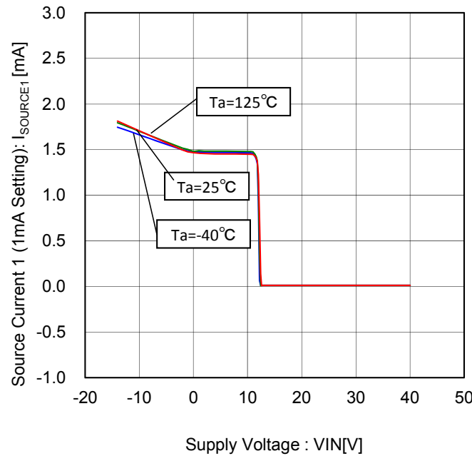
Figure 34. Source Current 1- Voltage Characteristic (1mA Setting)
