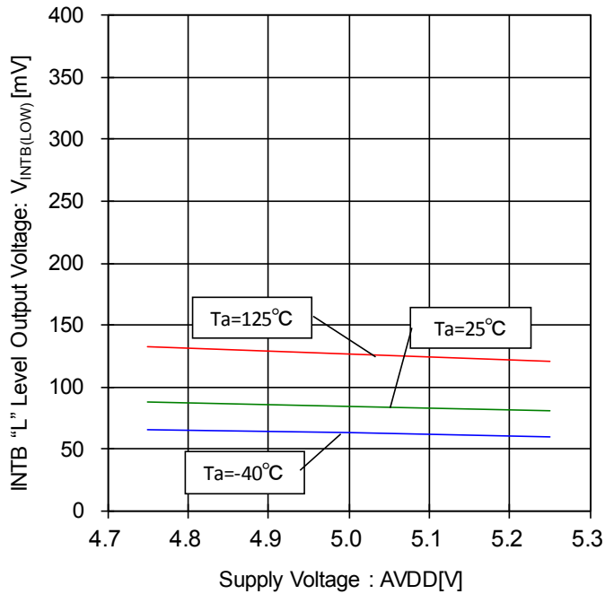
Figure 104. INTB "L" Level Output Voltage- Voltage Characteristic ( I_{SINK}=1.0\text{mA} )
