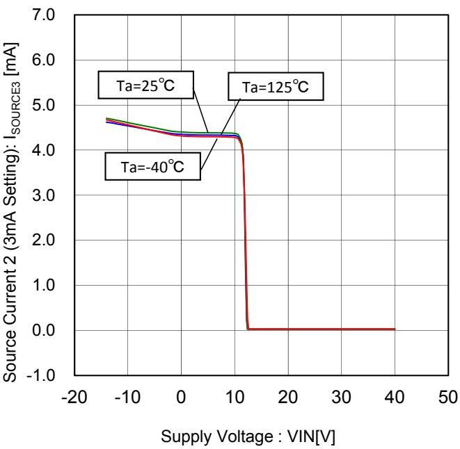
Figure 42. Source Current 2- Voltage Characteristic (3mA Setting)
