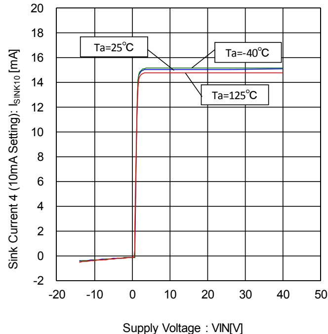
Figure 62. Sink Current 4- Voltage Characteristic (10mA Setting)
