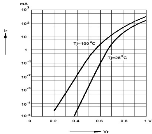
Figure 3. Forward Characteristics
