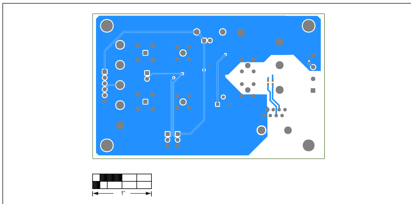
MAX22500E EV Kit—Bottom
