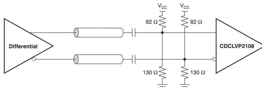
Figure 19. AC-Coupled Differential Inputs to CDCLVP2108 ( V_{CC} = 3.3 V)
