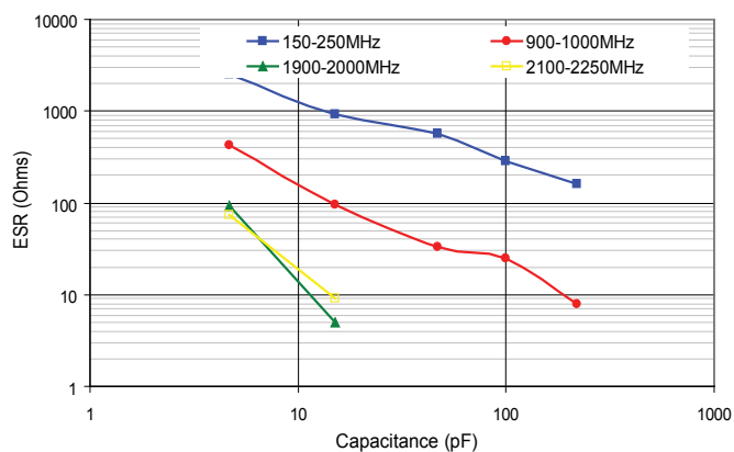
Q Factor: 0805/R15S
