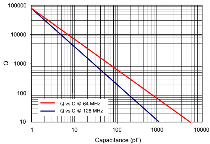
S48E Q vs. Capacitance, Typical (Preliminary)
