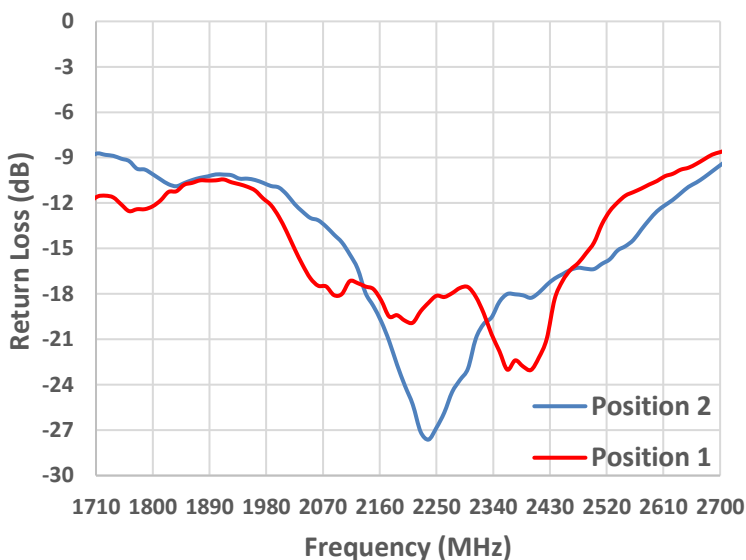
High Band Return Loss (1710 - 2700 MHz)
