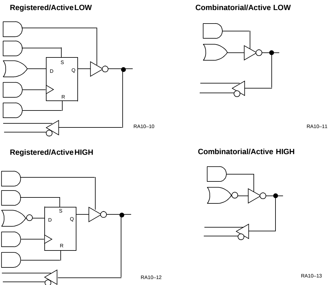
Figure 3. Four Possible Macrocell Configurations for the PLDC20RA10
